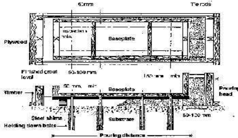
Shuttering detail 3: Metalation and grouting of base plates
